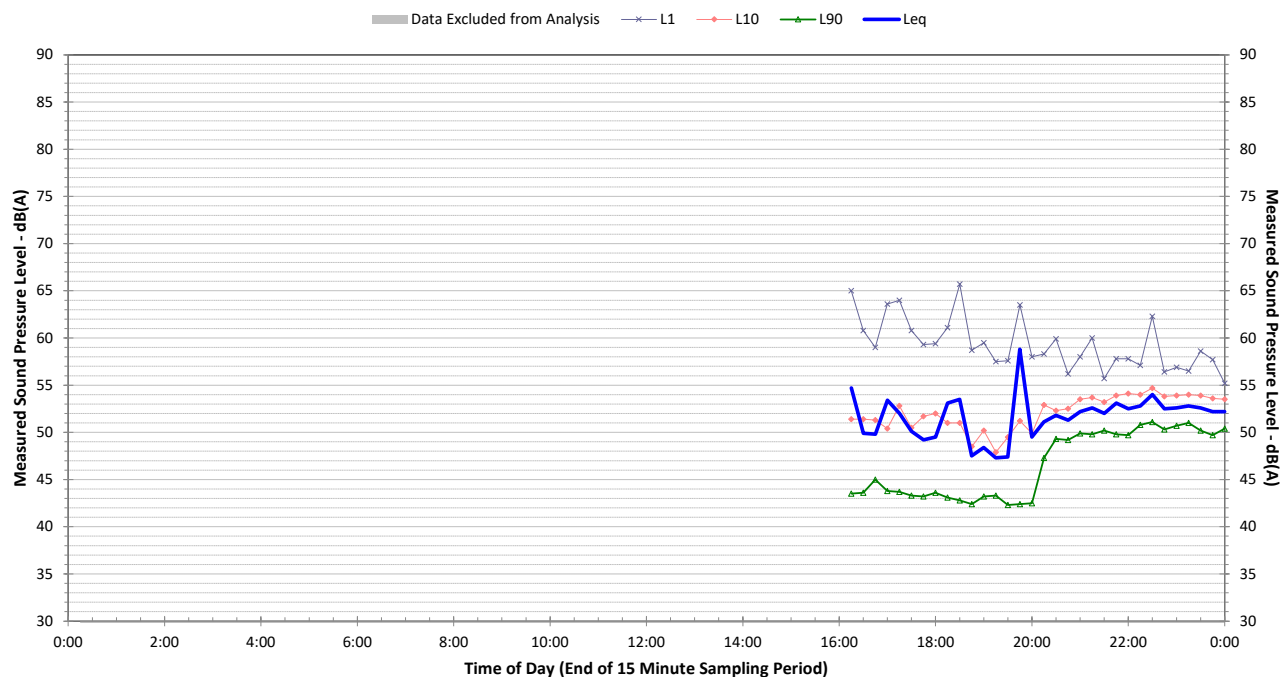
Profile of Noise Environment - Noise Monitoring Location 1 Thursday 26 November 2020
