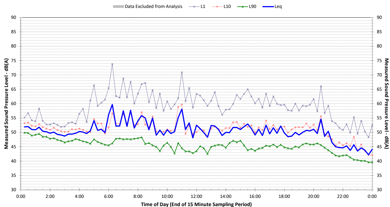
Profile of Noise Environment - Noise Monitoring Location 1 Friday 27 November 2020
