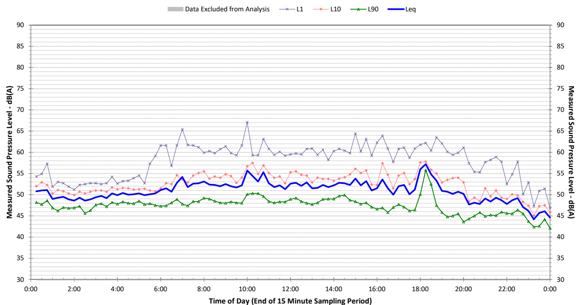
Profile of Noise Environment - Noise Monitoring Location 1 Tuesday 12 April 2022
