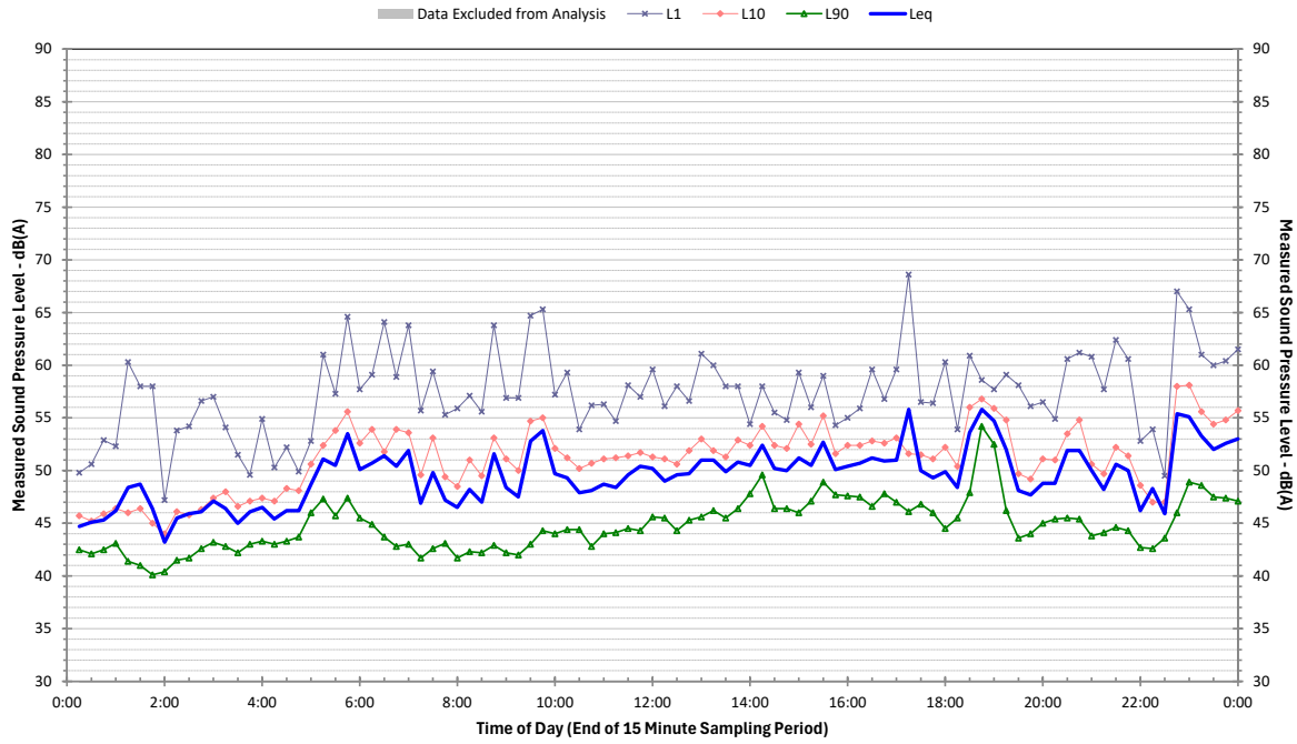
Profile of Noise Environment - Noise Monitoring Location 6 Tuesday 8 October 2024
