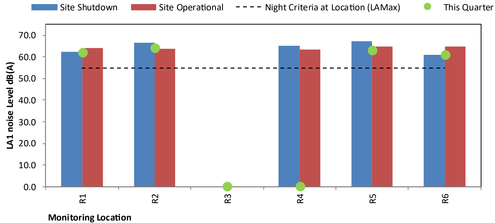
Figure 3-5: Long term LA1 noise levels at R1 – R6
